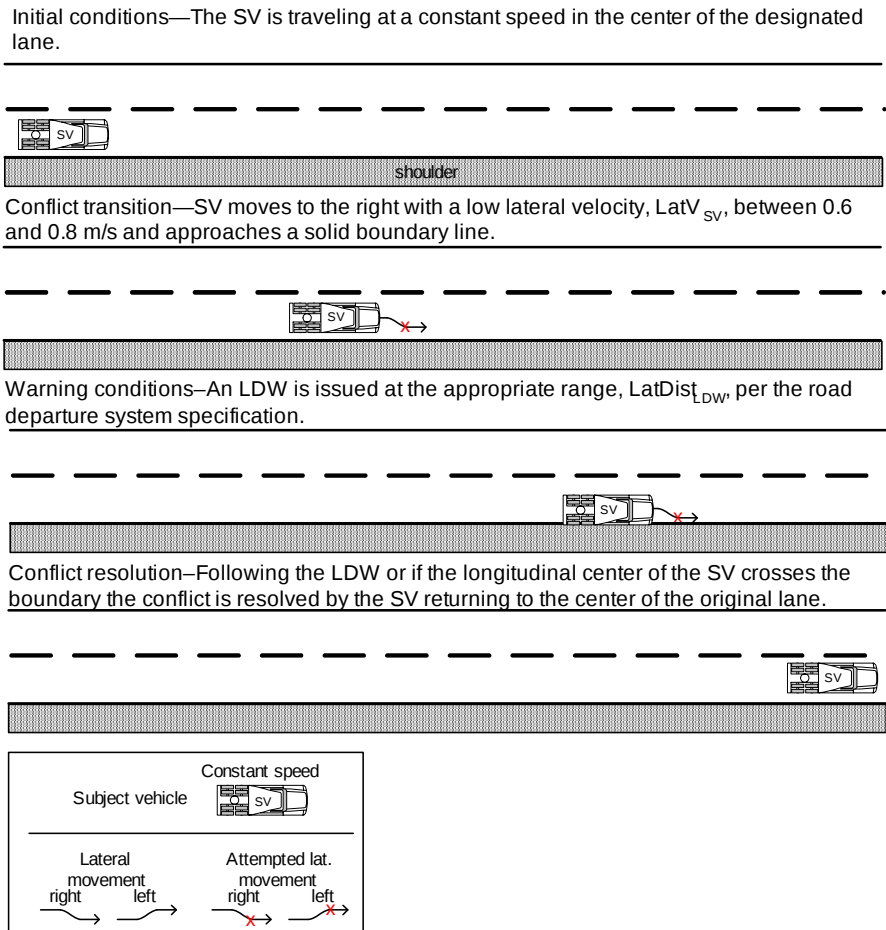
Figure 20. Test concept for road departure toward a clear shoulder with high lateral speed.
