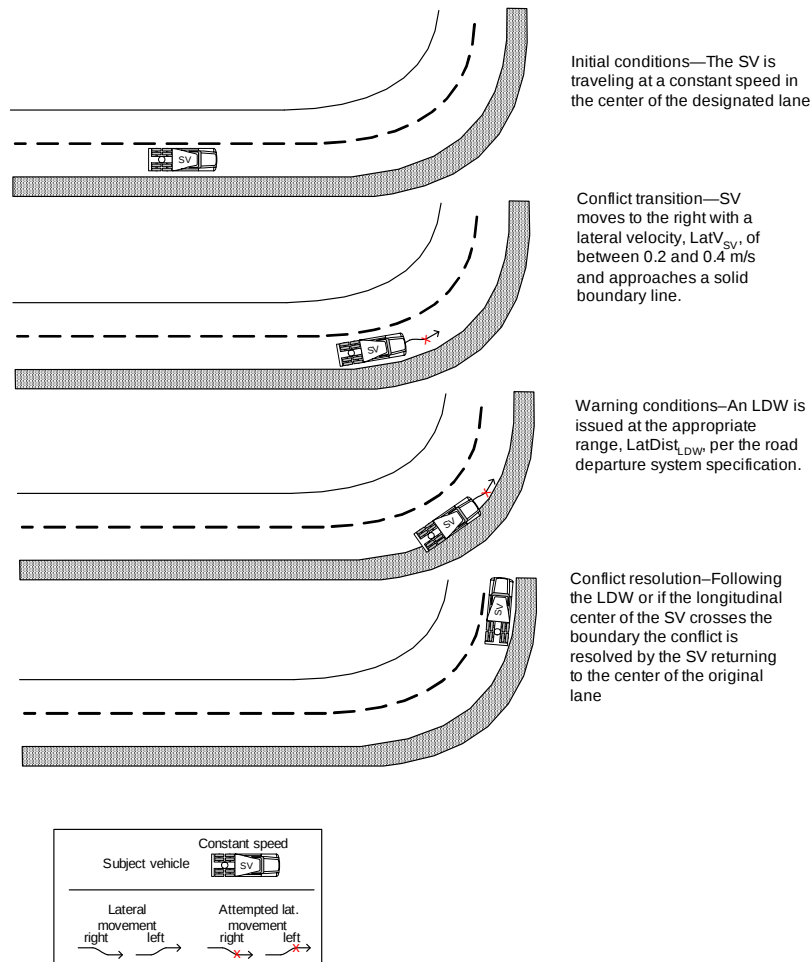
Figure 21. Test concept for road departure toward a clear shoulder on a small radius curve.
