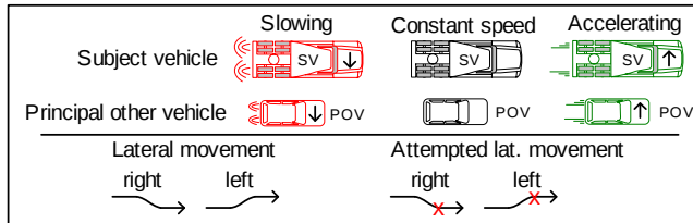
Figure 3. Test concept for rear-end conflict with a modestly slowing POV and a short time gap.
