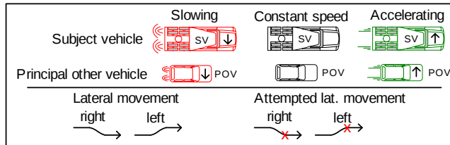
Figure 6. Test concept for rear-end conflict with slower POV after a lane change.
