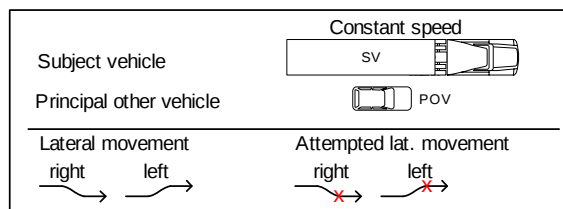
Figure 13. Test concept for lane-change conflict with POV in blind-spot (front bumper) on right.
