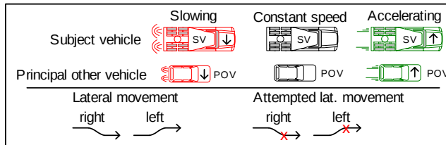
Figure 28. Test concept for a no-warn test when a faster POV cuts in front of the SV and separates.
