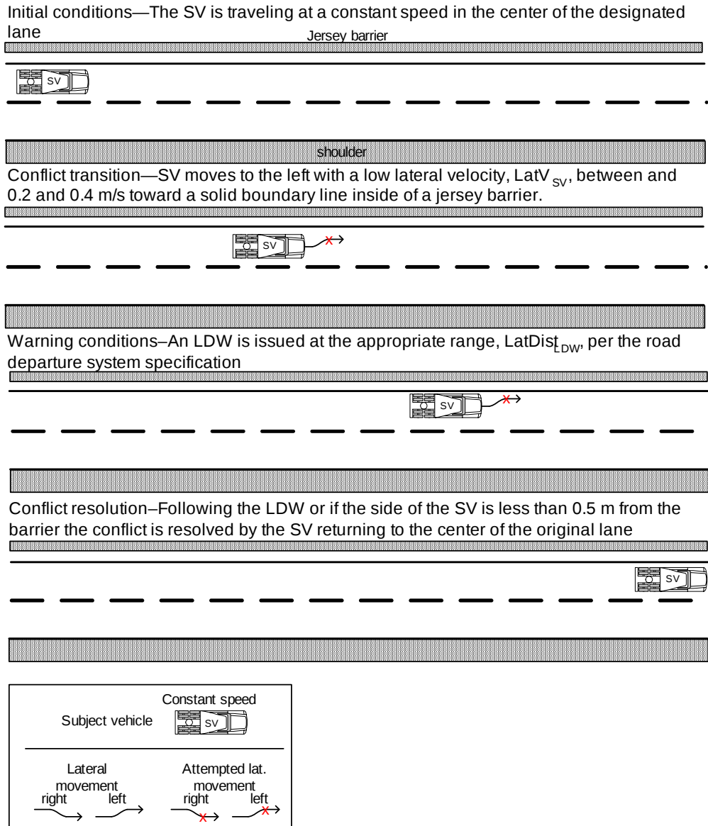
Figure 23. Test concept for road departure toward a barrier with no lane marker.
